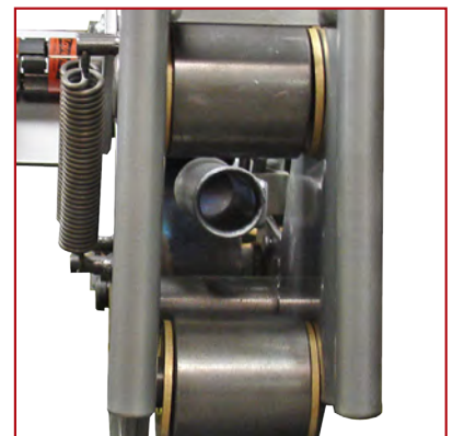
Self-Storing Fairlead
