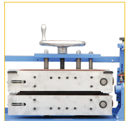
2" and 4" Capacity Pulling Heads
