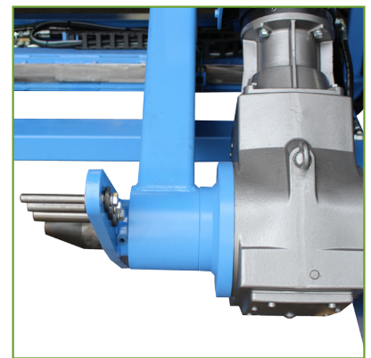
Drive Pins
