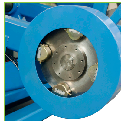
Multi-Caliper Holding Brake
