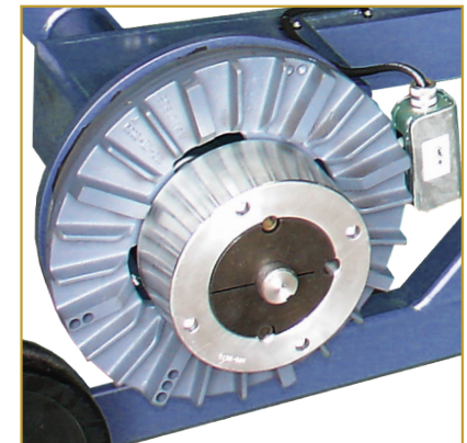
Pay-out Brake
