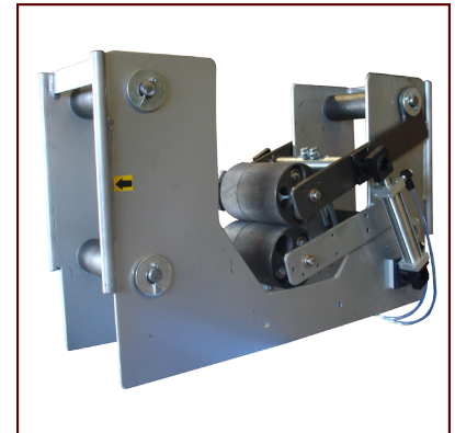
1706 with Pneumatic Cylinders
