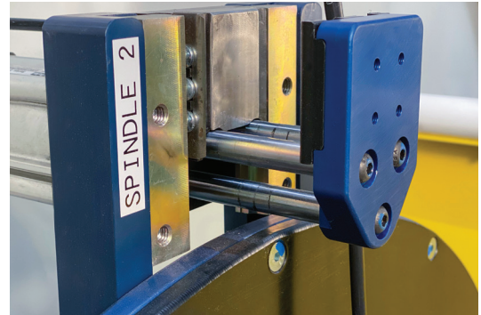
Integrated Gripper Cutter
