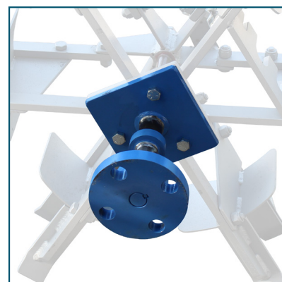
5C-6 Coiler with Slide Drive Adaptor
