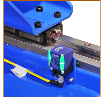
Traverse Safety Limits
