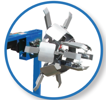
5C-6HD Collapsible Coiler 20" ID x 30" OD x 5" wide
